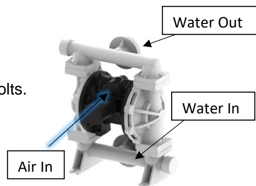
Figure 4.7-Chemical Transfer Pump
